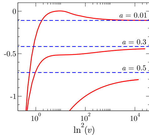
FIG. 5. Plot of \ln f_0(v)/\ln^2(v) following from (59), as a function of \ln^2(v) (increasing as v \rightarrow 0 ), for different values of a and g = 1 . To each set is associated a horizontal line marking the expected limit \chi/2 = (2 \ln a)^{-1} , see Eq. (69), from which we may see the approach toward the limit becoming extremely slow as a increases.
