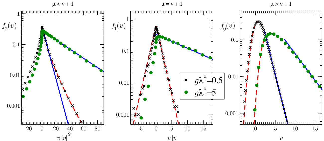
FIG. 2. Asymptotic behavior in a Gaussian bath ( \mu = 2 ). From left to right: f_2(v) , f_1(v) and f_0(v) , computed from DSMC simulations for a = -1/3 , g = 1 (crosses) and a = 1/3 , g = 3 (dots). The solid line is the cold bath behavior f_\nu(v) \propto \exp[-v|v|^\nu/(\nu+1)g] , while the dashed line is the "equilibrium" asymptotic f_\nu(v) \propto \Phi(\lambda v) which always describes the left tail ( v \rightarrow -\infty ). For f_2(v) (left), the same asymptotic expression describes the right tail, although the value of the threshold v_c = g\lambda^\mu may be too high for the crossover to be easily observable (as seen here with the dots which retain the cold bath behavior for the whole velocity range reported).
