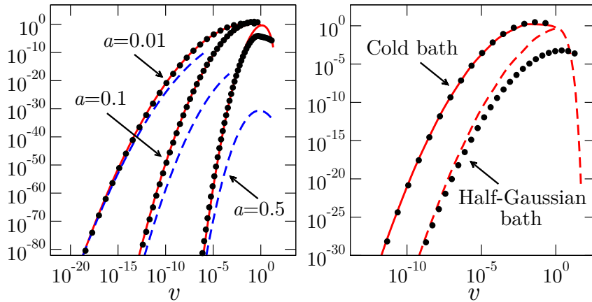
FIG. 6. Left: Validity of the asymptotic expressions. The exact cold bath solution f_0(v) [solid lines, corresponding to (59)] against the predictions (69) (dashed lines) and (85) (dots). Here, a = 0.01, 0.1 and 0.5 from left to right, and g = 1 . As a increases, the predicted asymptotic behavior appears further in the tail, and the expansion (85) becomes significantly more precise than our first heuristic guess (69). Right: Close-up on the data for a = 0.01 (solid line) and comparison with the solution corresponding to a half-Gaussian bath \Phi(v) = \Theta(v)(2\pi)^{-1/2} \exp(-v^2/2) (dashed line), other parameters being identical. The same asymptotic form (85) (dots) holds in both cases. Similar behavior is expected for any bath distribution with a lower velocity bound, provided g > 0 and a > 0 .
