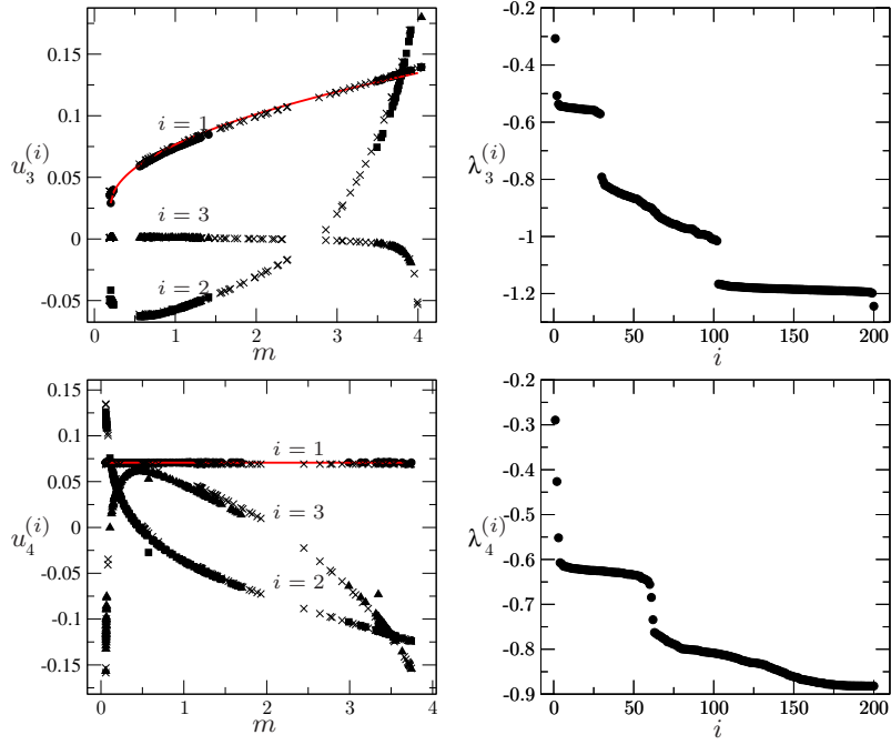
FIG. 4. The three eigenvectors associated with the three largest eigenvalues (left) and the eigenvalue spectrum (right) for n = 3 (top) and n = 4 (bottom) for the optimal dispersion c(m) reported in Fig. 3. The index i ranks the eigenvalues in decreasing order. Concerning the eigenvectors: crosses are obtained from Method A and full symbols from Method B discussed in section IV A. No symbols are reported for masses such that c(m) = 0 , hence the gaps in the data. The solid lines correspond to the ansatz u_3^{(1)}(m) \propto \sqrt{m - m_-} (with m_- the minimal mass in the system) and u_4^{(1)}(m) \propto 1 . Only the second one illustrates the dynamical equipartition property alluded to in section III.
