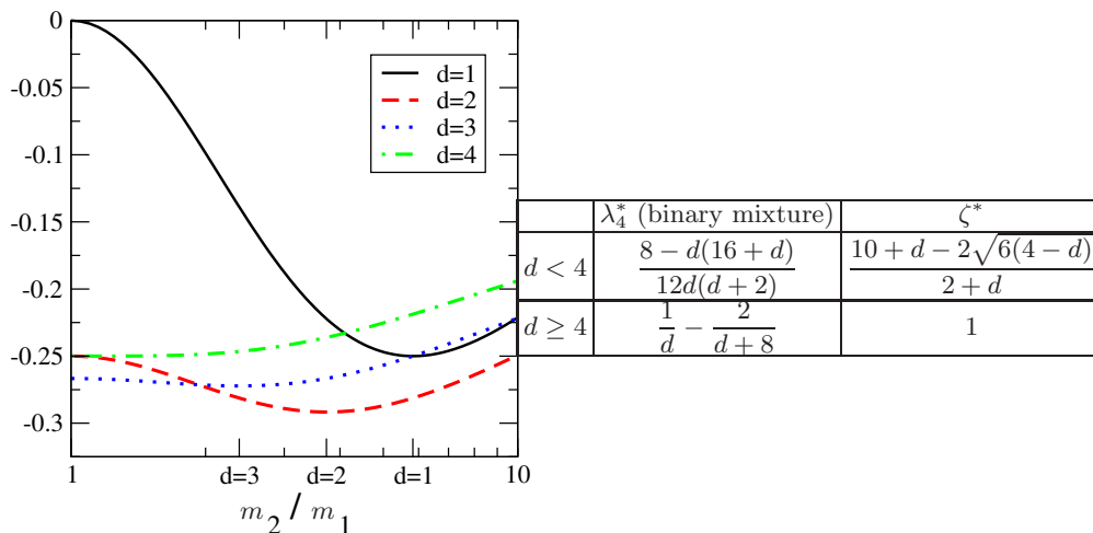
FIG. 5. Left: Relaxation rate for the d -dimensional Sonine moment \langle S_n(mv^2/2) \rangle of an equimolar binary mixture, in dimension d = 1 up to 4. The locations of the optimal mass ratios are marked on the x -axis for d < 4 : although relaxation is possible in the monodisperse case \zeta = 1 for any d > 1 , there remains a polydisperse optimum until d = 4 . Right: Optimal relaxation rate and corresponding mass ratio for a binary mixture in arbitrary dimension d (it is necessarily equimolar due to the symmetries of the operator).
