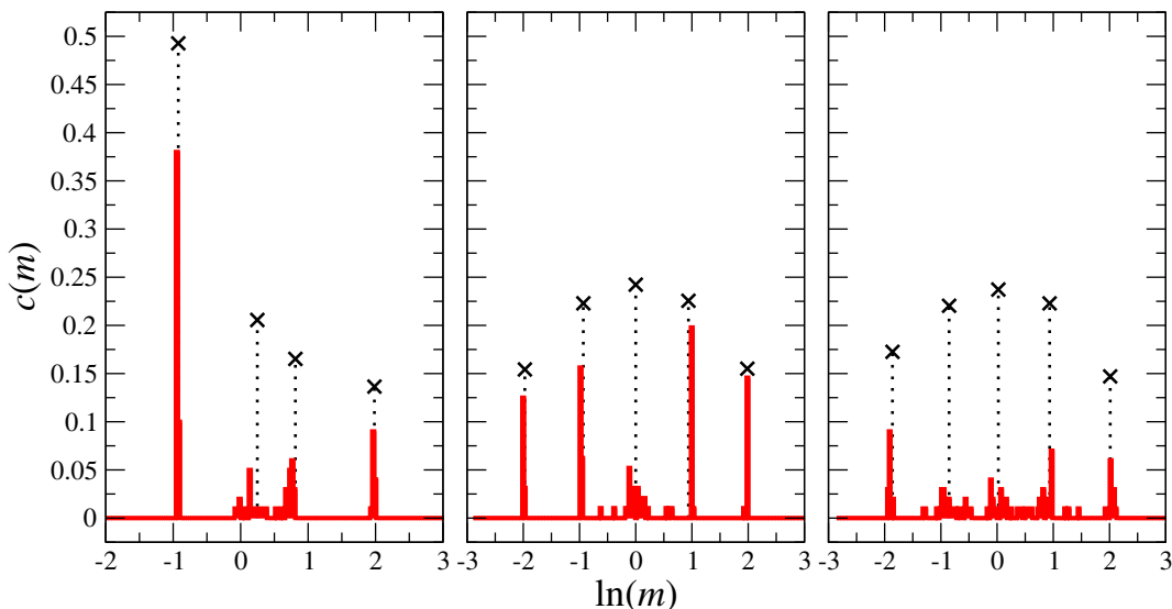
FIG. 3. Mass distributions optimized for \lambda_3^* (left), \lambda_4^* (center) and the composite eigenvalue \lambda^* (right) corresponding to the true optimum (17) for one-dimensional Maxwell molecules, i.e. \nu = 0 in equation (7). The crosses represent the optimal mixtures with a few species, either N = 4 or N = 5 and the mean mass fixed to unity (their abscissae are reported with dashed lines). The histograms are for a "continuous distribution" approximated with N = 200 species, methods A and B giving equivalent results. We see that the continuous case is an approximation of the few-species mixture, and that the optimum for the composite eigenvalue is very close to that of \lambda_4 – although its minimization is more difficult due to its singularity, and leads to a larger spread in the continuous approximant. Note that for n = 4 (center), c^*(m) is an even function of \log(m) , up to a trivial shift, which illustrates the invariance under m \rightarrow 1/m .
