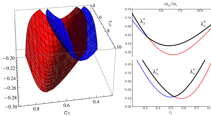
FIG. 2. Crossing of \lambda_3^+ and \lambda_4^+ . Left: graphs of both eigenvalues against concentration c_1 and mass ratio \zeta = m_2/m_1 . Right: section view of these surfaces for c_1 = 0.6 (top) and \zeta = 4 (bottom). The longest-living mode is highlighted in bold: it is the mode n = 3 on the left of the intersections, and n = 4 on the right. In principle, optimizing the relaxation involves finding the minimum of the composite curve (or surface) defined by the highest mode at each point.
