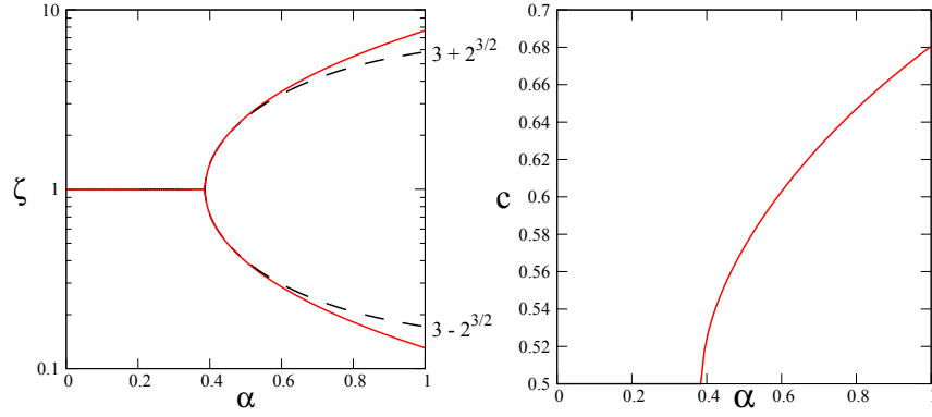
FIG. 8. Optimization of \lambda_3^+ in the (forced) binary mixture with finite restitution coefficient \alpha \in [0, 1] . The dashed branch ending at 3 \pm 2\sqrt{2} shows the equimolar result, while the more general solution allowing for unequal concentrations is shown with the continuous curve. The corresponding values of \zeta = m_2/m_1 and c_1 are found to vary continuously from the elastic limit \alpha = 1 to the threshold \alpha_c \approx 0.37 , where the optimum becomes the single-component gas m_2 = m_1 . This bifurcation does not appear for the rescaled eigenvalues of the free cooling state.
