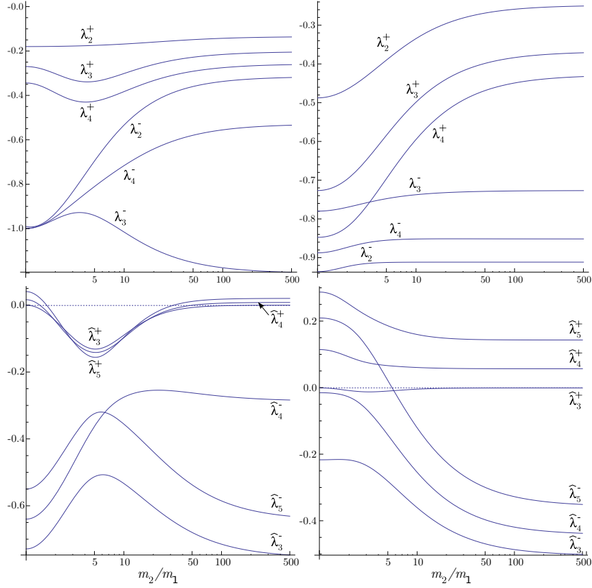
FIG. 7. Eigenvalues spectrum for the inelastic equimolar binary mixture versus mass ratio, with \alpha = 0.8 (left) and \alpha = 0.2 (right). Top: spectrum in the forced state. Bottom: rescaled eigenvalues in the free cooling state (the dotted line materializes the ordinate 0 allowing to see all eigenvalues that cross it, representing diverging moments).
