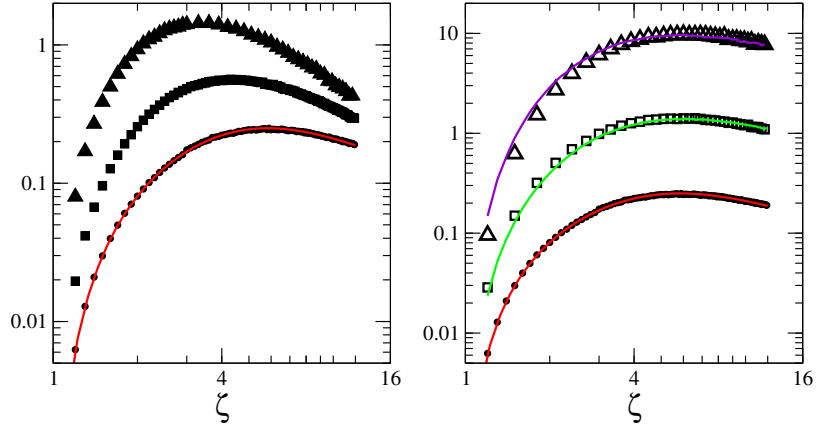
FIG. 6. Relaxation rate of the fourth moment for different collisions kernels \nu = 0, 1, 2 (circles, squares, triangles) in an equimolar binary mixture, fixing either the velocity scale (left) or the temperature and mean mass (right). For Maxwellian particles \nu = 0 , both constraints give the same result |\lambda_4^+| (solid line, left picture). However, for hard or very hard particles ( \nu = 1, 2 ) the choice of constraints displaces the maximum through a change of scale: the data in the first picture are multiplied by m^{\nu/2}1.2^\nu to give the solid lines in the second (the numeric factor is adjusted by fit). The constraint of fixed temperature and mean mass leads to all three models exhibiting optimal mass ratios within ten percent of each other.
