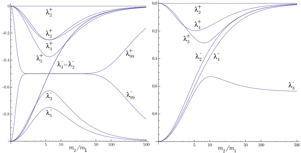
FIG. 1. Eigenvalue spectrum of the operator acting on U^n on the right-hand side of Eq. (11), for a binary mixture, as a function of mass ratio \zeta = m_2/m_1 . Left: equimolar case c_1 = 1/2 , all the extrema with \zeta \neq 1 are aligned at \zeta = 3 + 2\sqrt{2} ; let us note that in this case \lambda_2^- = \lambda_4^- = -4\zeta/(1 + \zeta)^2 . Right: c_1 = 0.68 , the extrema are displaced and \lambda_3^+ and \lambda_4^+ now cross.
