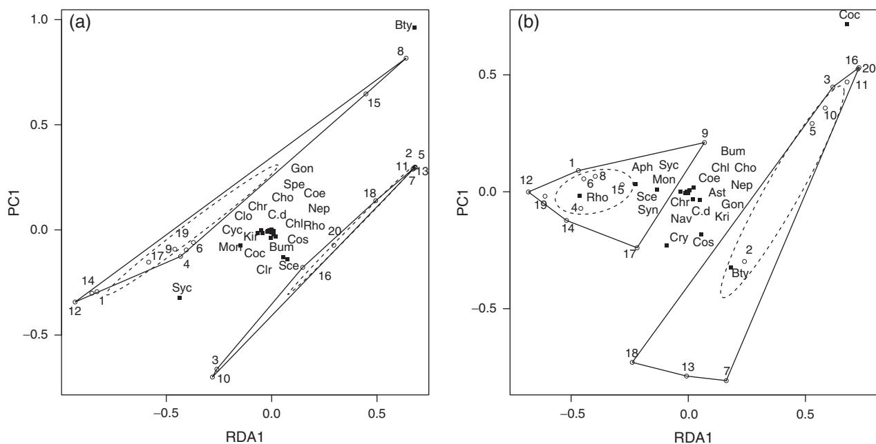
Fig. 3 Redundancy analysis (RDA) biplot for sites (i.e. mesocosms) and species scores for phytoplankton taxa recorded in the mesocosm experiment in April (a) and October (b). In both cases, RDA 1 was constrained by treatment and accounted for 24.1% and 24.6% of the variation in the taxonomic composition of the mesocosms in April and October, respectively. In the plot, the dotted lines denote the 95% confidence ellipses around the centroids for both treatments. In both April and October, these ellipses do not overlap indicating that the community composition was significantly different between warmed and ambient treatments. The solid lines enclose all mesocosms that belong to a particular treatment; in both cases heated treatments (1, 4, 6, 8, 9, 12, 14, 15, 17, 19) cluster to the left, whereas ambient treatments (2, 3, 5, 7, 10, 11, 13, 16, 18, 20) cluster to the right. Genus abbreviations are as follows: Aphanothece (Aph), Asterococcus (Ast), Botryococcus (Bty), Bumilleriopsis (Bum), C.dinobryonis (C.d), Chlorella (Chl), Chlorococcum (Coc), Chroococcus (Chr), Chroomonas (Cho), Coenococcus (Coe), Cosmarium (Cos), Cryptomonas (Cry), Goniocloris (Gon), Kirchneriella (Kri), Monoraphidium (Mon), Navicula (Nav), Nephrocytium (Nep), Rhodomonas (Rho), Scenedesmus (Sce), Synechococcus (Syn), Synechocystis (Syc), Spermatozopsis (Spe).
